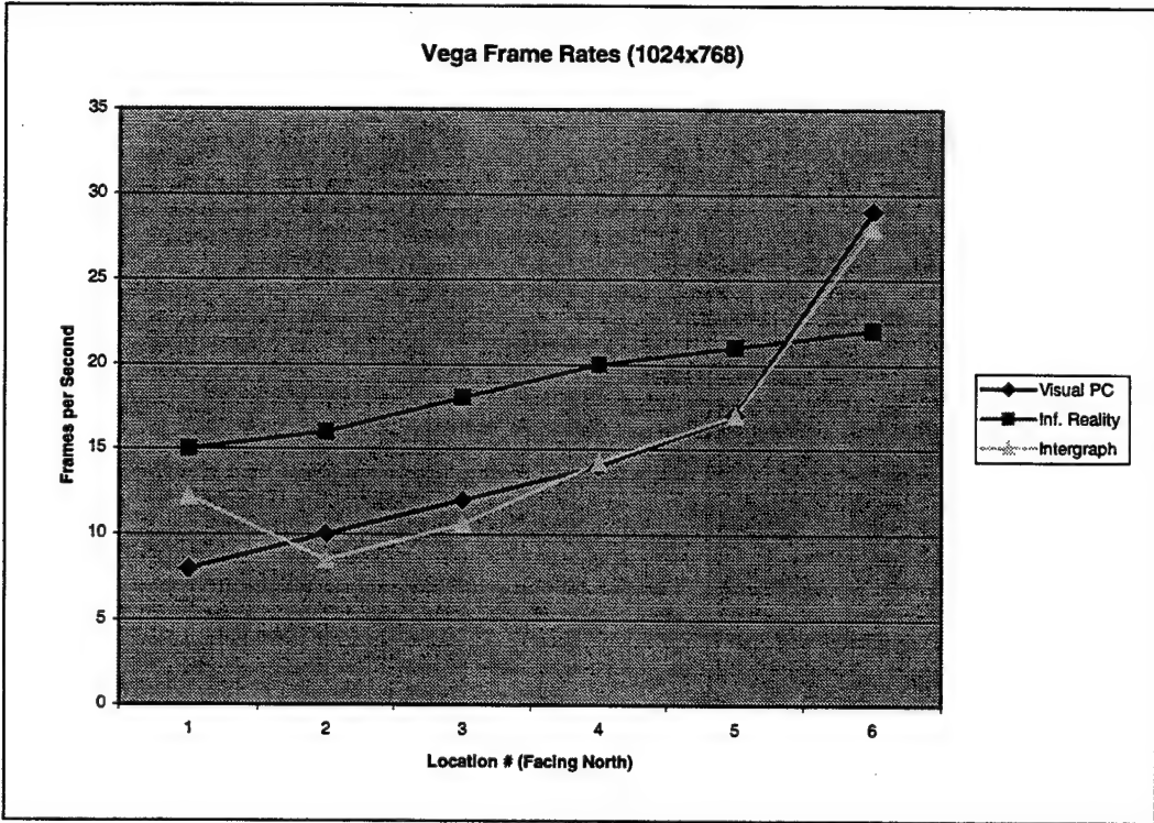
Figure 6.5. Performance graph of Vega facing North.
